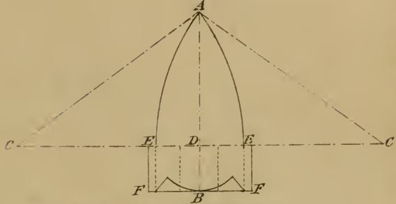
No. 6 Perfect shape for Rifle Balls.
